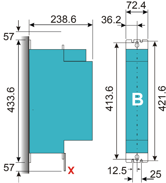
Dimensions are in millimeters (X : Power Bracket - 890 Installation Kit)
