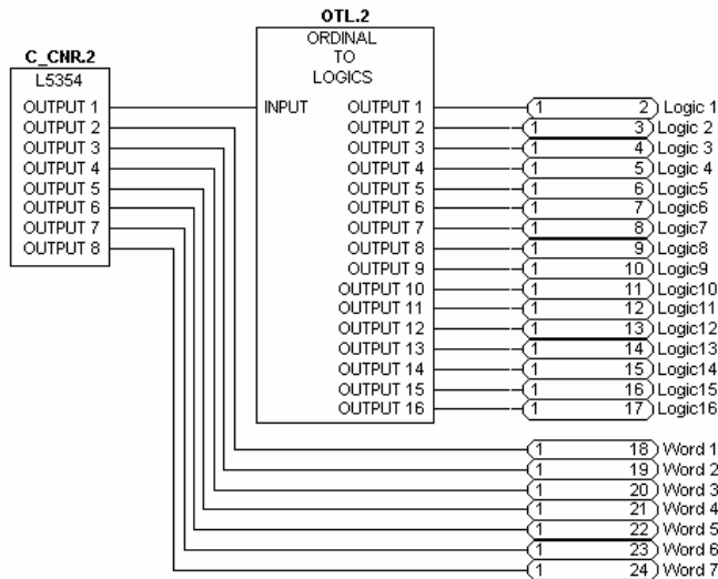
Figure 7. Ordinal to Logical and Value LINK Setup
