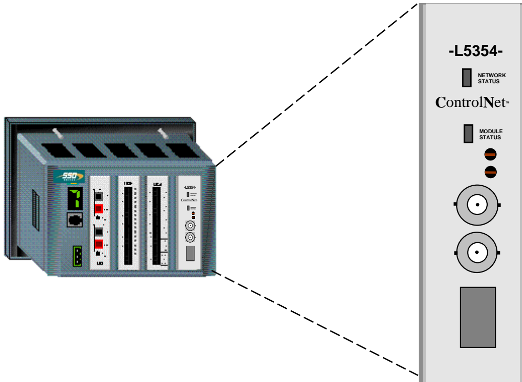
Figure 1. L5392 LinkStation with L5354 ControlNet LinkCard
