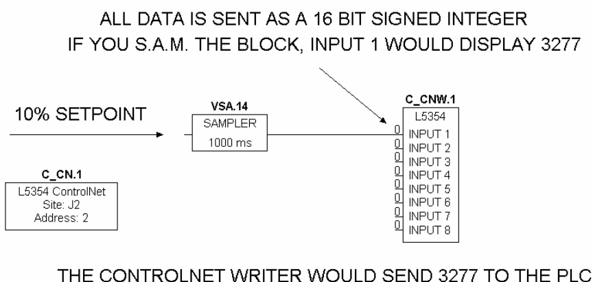
Figure 5. Basic LINK Setup
