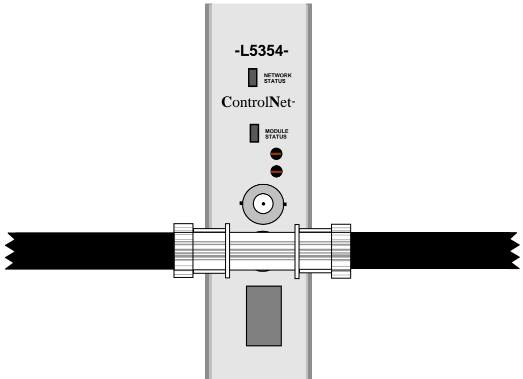
Figure 3. ControlNet connections to the L5354
