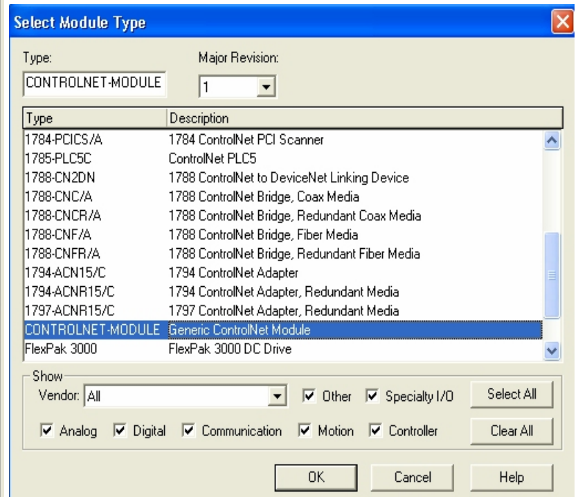
Figure 11. Select Remote Module Type
