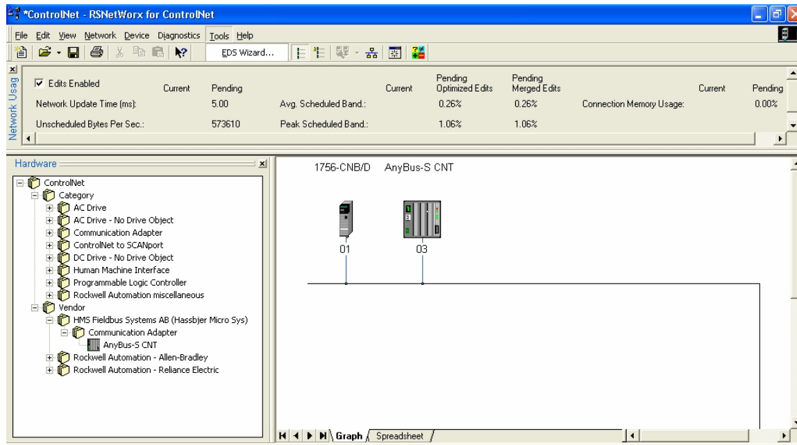
Figure 15 RSNetworkx configuration screen
