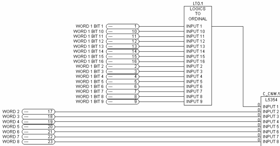
Figure 6. Logical to Ordinal and Value LINK Setup
