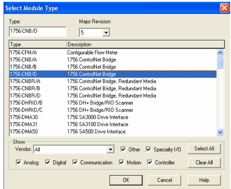
Figure 9. Select Scanner
