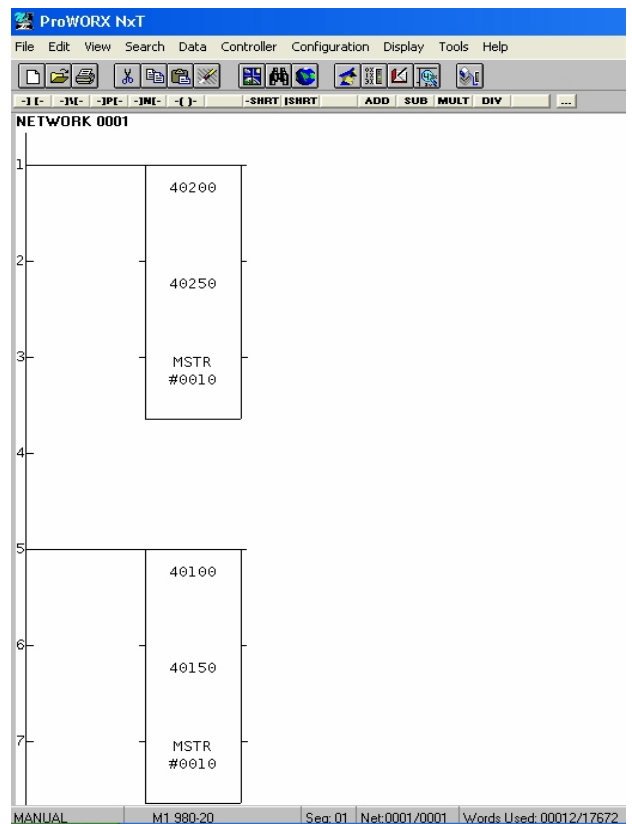
Figure 6 PLC Ladder Logic Showing MSTR Blocks
